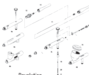
Revolution Airbrush Parts
