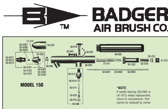
Model 150 Airbrush Replacement Parts (Qty=Each)
