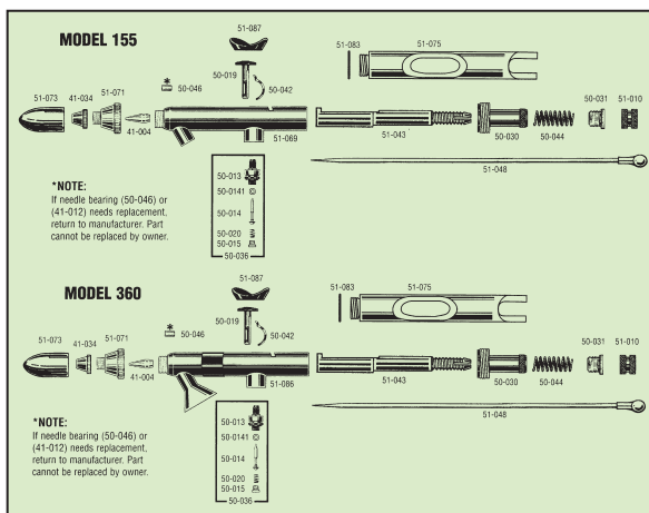
Model 155/360 Airbrush Replacement Parts (Qty=Each)
