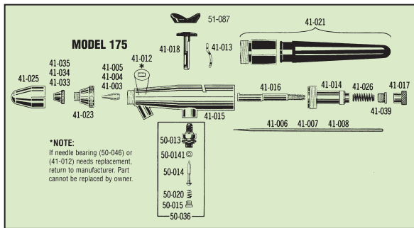
Model 175 Crescendo Airbrush Replacement Parts (Qty=Each)
