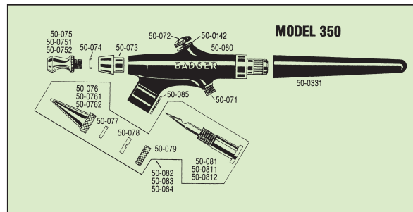
Model 350 Airbrush Replacement Parts (Qty=Each)
